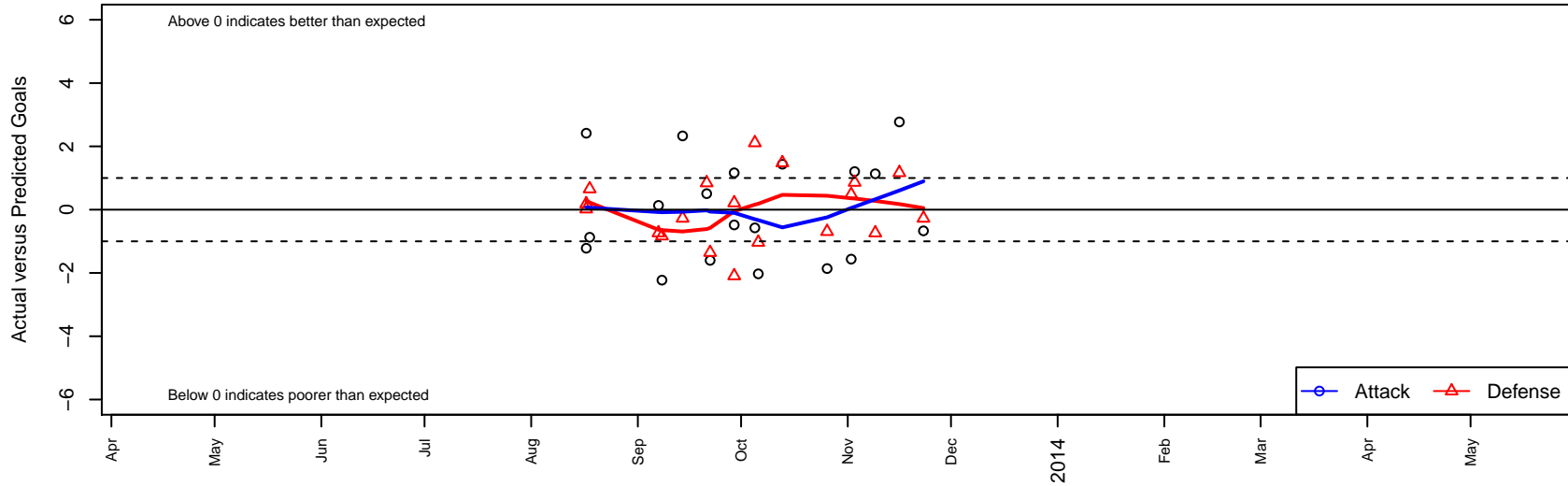
Exiles SC Black B02 Dots are actual minus expected GF (blue circles) and GA (red triangles). Blue line is smoothed change in attack strength. Red is smoothed change in defense strength.
